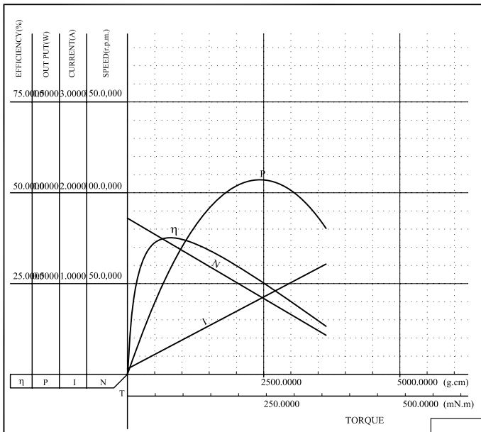
MODEL:DS-13SS05000513000-150K VOLTAGE: 5.0V
