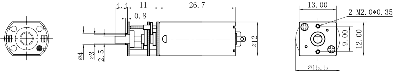
MODEL:DS-13SS05000513000-150K VOLTAGE: 5.0V
