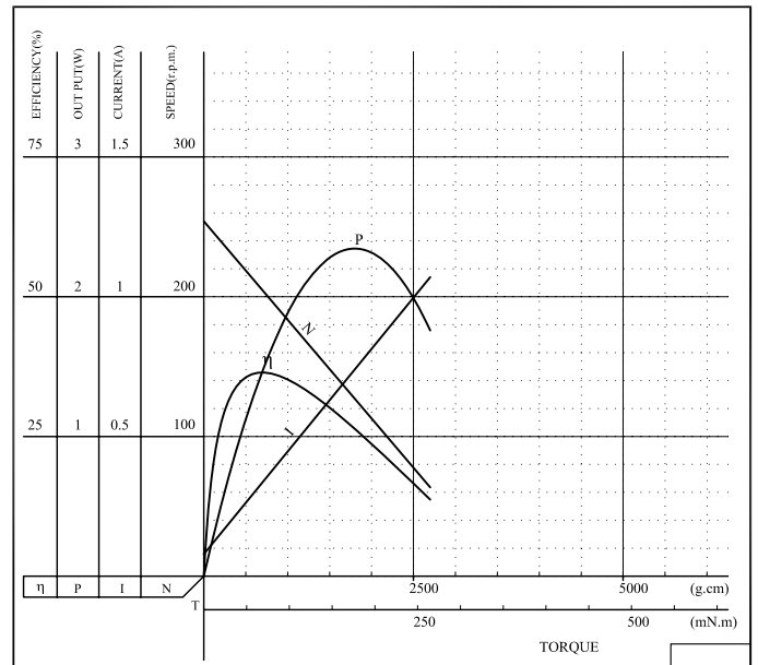
MODEL:DS-13SS05001216000-63K VOLTAGE: 12V
