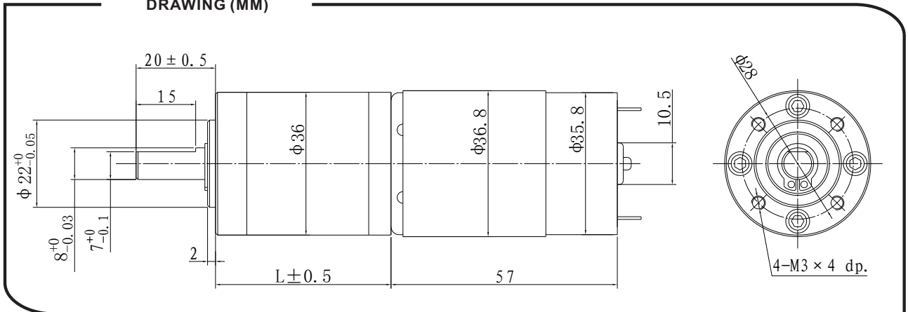
DRAWING (MM)
