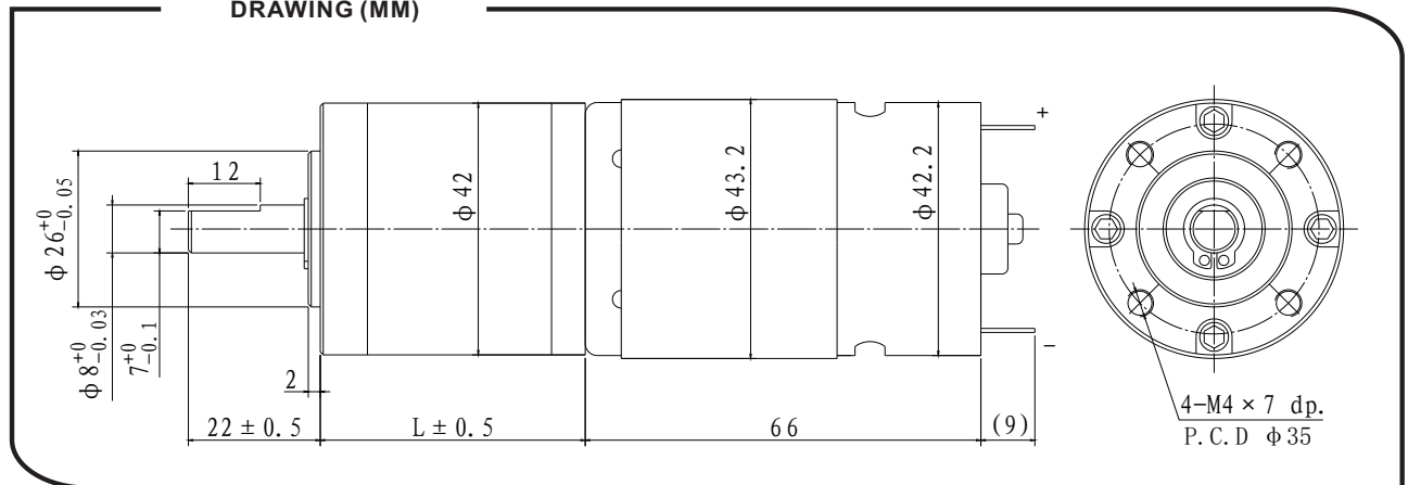
DRAWING (MM)
